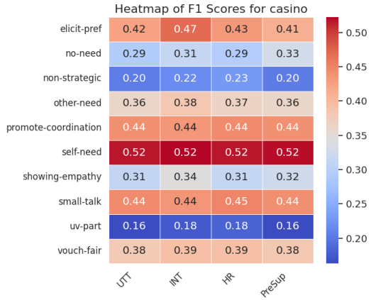
(a) Casino
