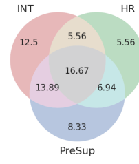
(c) res_CB
