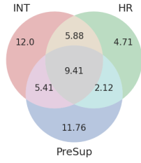
(a) CaSiNo
