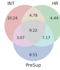
(c) res_CB
