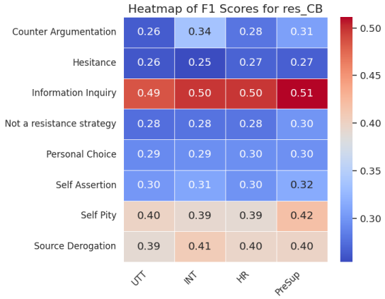
(c) res_CB
