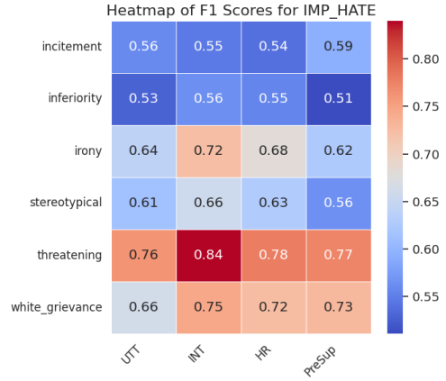
(f) IMP_HATE
