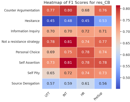
(c) res_CB
