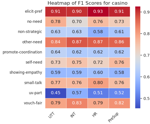
(a) Casino
