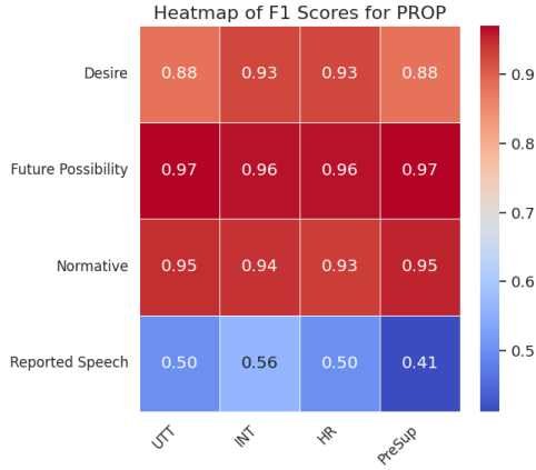
(e) PROP
