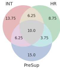
(a) CaSiNo
