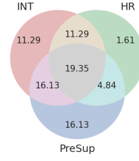
(f) IMP_HATE
