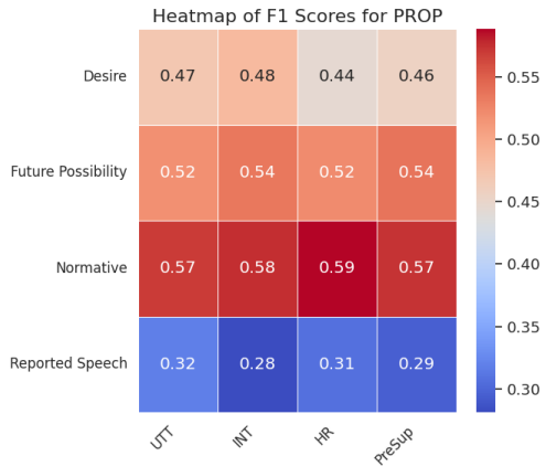
(e) PROP
